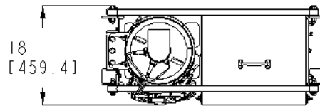
Figure 3-12.1 Side View —Model 220 CRP Laden Height and Length Measurement
