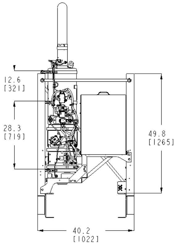
Figure 3-12.2 Model 220 Vertical Exhaust Measurement inches (mm)
